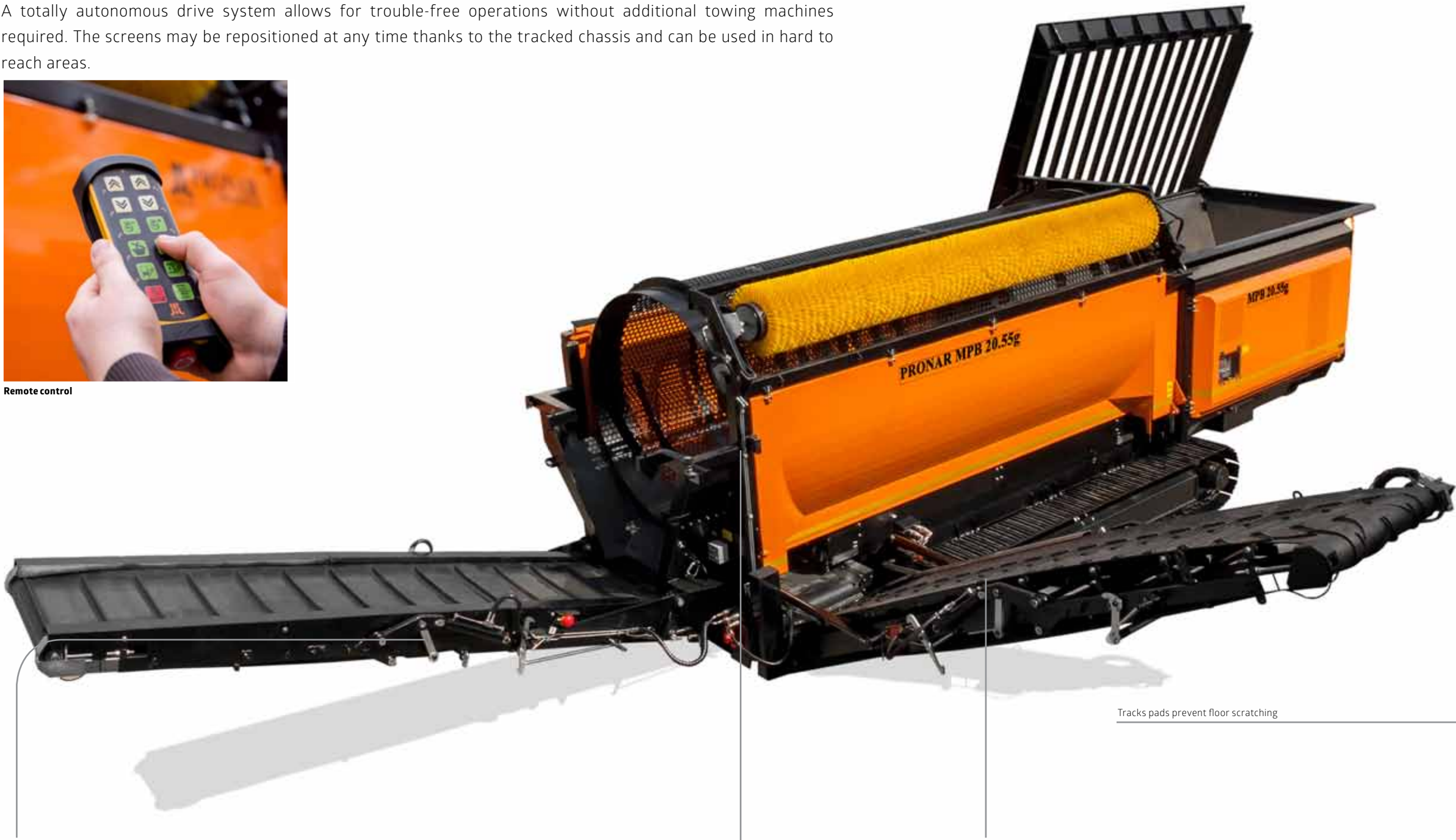
Rear conveyor folded by means of two hydraulic cylinders
