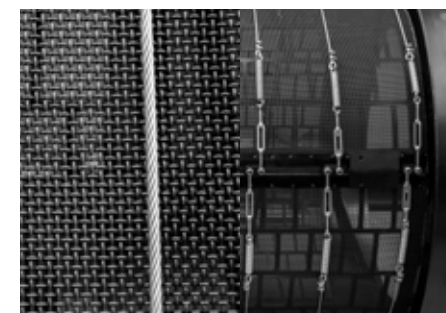
Special mesh drum for perforation <10mm
