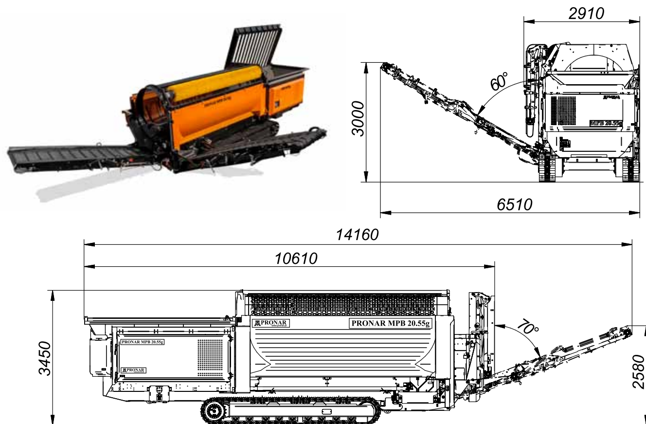
Tracked mobile trommel screen MPB 20.55g
