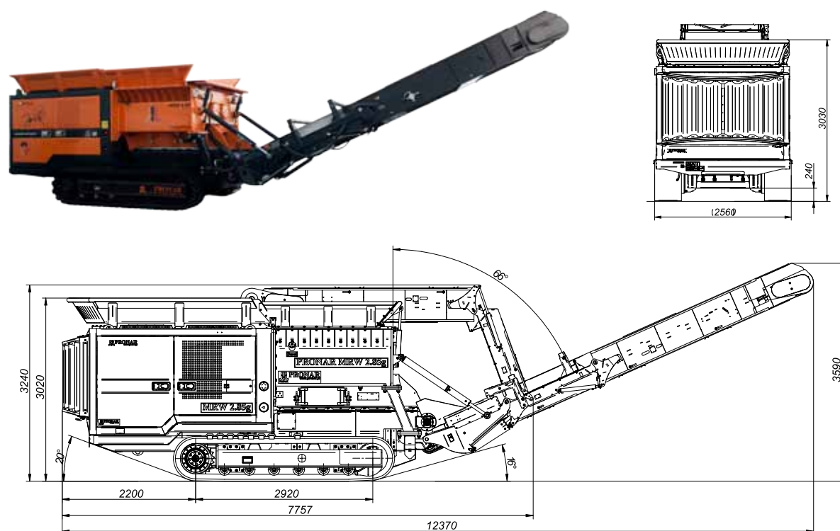
Mobile slow-speed shredder on tracked chassis MRW2.85g
